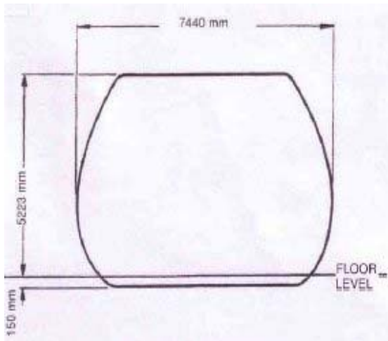
Mk 4 excavation profile
